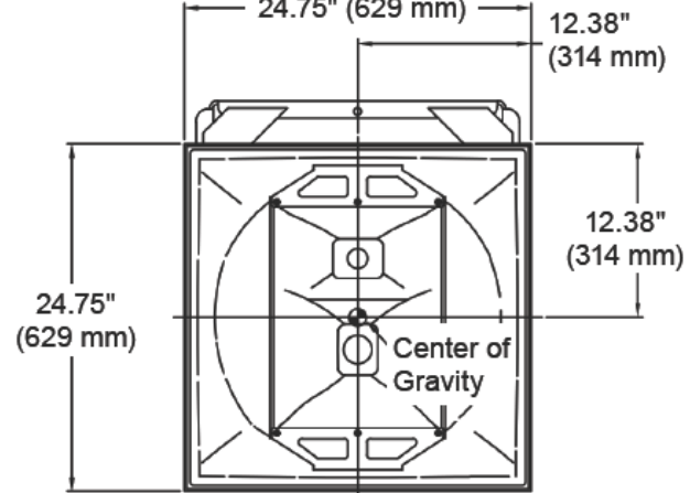
Front
