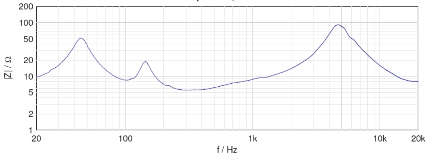
Impedance, 1/6 Oct.
