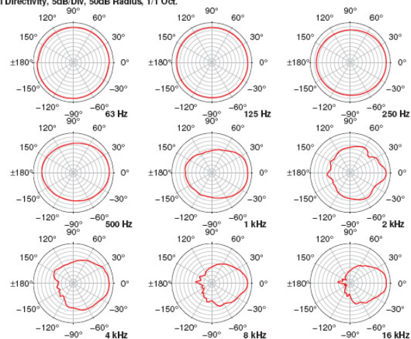
Vertical Directivity, 5dB/Div, 50dB Radius, 1/1 Oct.
