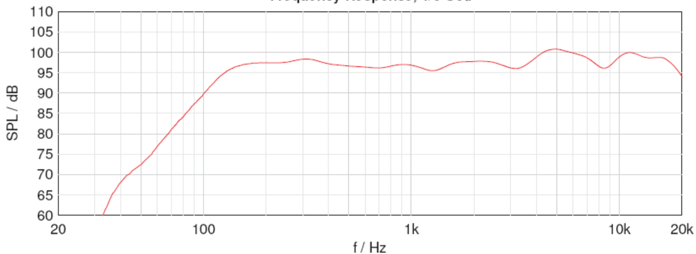
Frequency Response, 1/6 Oct.
