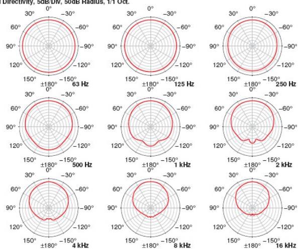
Horizontal Directivity, 5dB/Div, 50dB Radius, 1/1 Oct.
