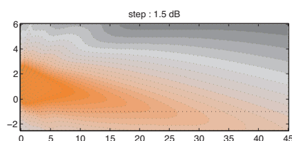
Step Array SA250P vertical directivity: sound level for the speech octaves (500Hz-1kHz-2kHz) in the vertical median plane.
