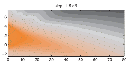
Step Array SA400P vertical directivity: sound level for the speech octaves (500Hz-1kHz-2kHz) in the vertical median plane.
